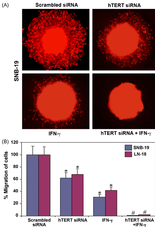
Fig. 3. Determination of migration of SNB-19 and LN-18 cells from spheroids after transfection with hTERT siRNA or treatment with IFN- \gamma or both agents together for 48 h. (A) Representative inhibition of SNB-19 cell migration from spheroids. Spheroids were prepared from SNB-19 control and treated cells stably expressing cGFP, transferred to a 24-well chamber, and allowed to migrate for 24 h. The migration of cells from the spheroids were observed under a fluorescent microscope and photographed. (B) Percentage of migration of SNB-19 and LN-18 cells from the center of the spheroids to the monolayers. The data are presented as mean \pm SD of 6 independent experiments from each group (* p < 0.001 compared with the control mean values and # p < 0.001 compared with hTERT siRNA or IFN- \gamma mean values).
